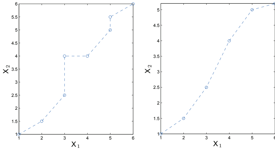
Figure 3: Comonotonic support (left panel) for a couple (X_1, X_2) and a strict comonotonic support (right panel) for a couple (X_1, X_2) .
