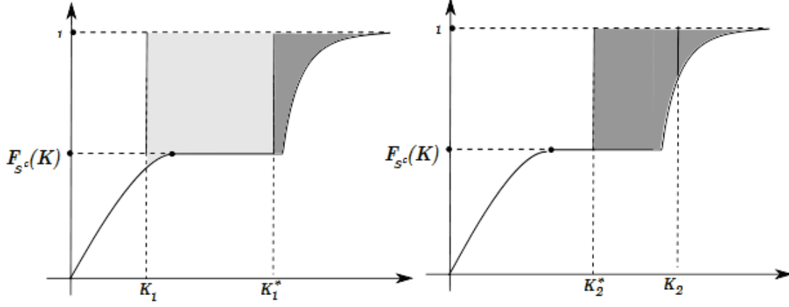
Figure 2: F_{X_1} (on the left), F_{X_2} (on the right), K \notin A , w_1K_1 + w_2K_2 = K and F_{X_1}(K_1) < F_{S^c}(K) .
